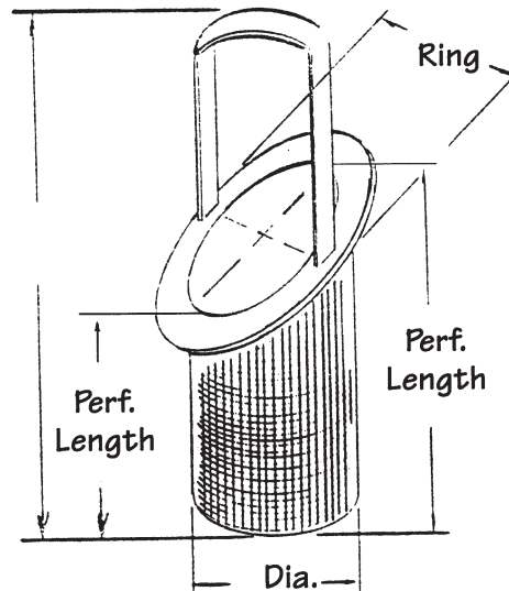
Basket Strainer
